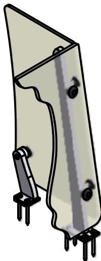
TYPICAL END PANEL SUPPORT CONFIGURATION
